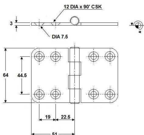
Code no. 60-06002 STAINLESS STEEL HINGES L 64 x W 102 x 3 mm
