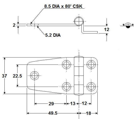
Code no. 60-06016 STAINLESS STEEL BUTT HINGES L 37 x W 67.5 x 2 mm
