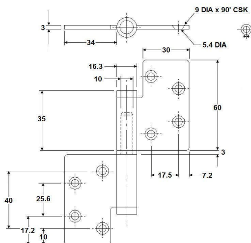
Code no. 60-06017 STAINLESS STEEL LIFT OFF HINGES
