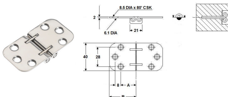
Code no. 60-06014 STAINLESS STEEL TABLE HINGES
