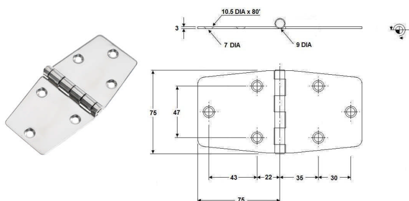
Code no. 60-06011 STAINLESS STEEL HINGES L 75 x W 150 x 3 mm
