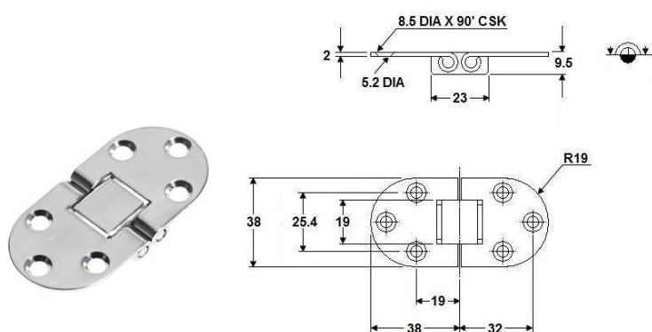
Code no. 60-06015 STAINLESS STEEL TABLE HINGES L 38 x W 76 x 2 mm
