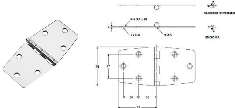
Code no. 60-06010 STAINLESS STEEL HINGES L 75 x W 150 x 2 mm
