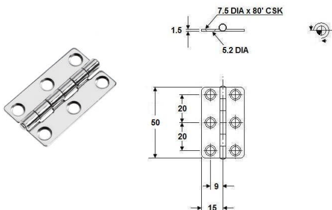
Code no. 60-06013 STAINLESS STEEL BUTT HINGES L 50 x W 30 x 1.5 mm
